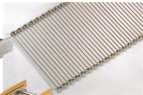
Nastro ad anelli Closed ring rod bars
