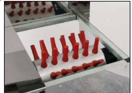
Aluminium roller with bigger diameter and 54 fingers for a quicker and effective plucking
